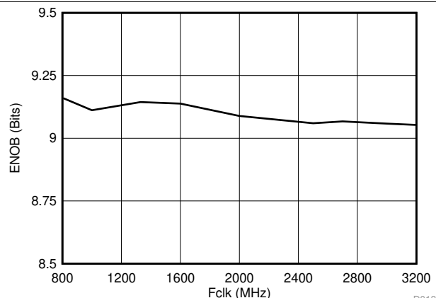
Figure 14. ENOB vs Clock Frequency
